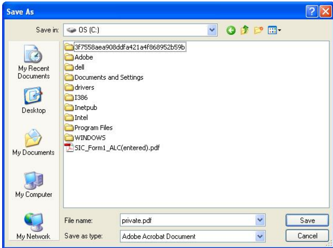
Figure 7 Windows browser
